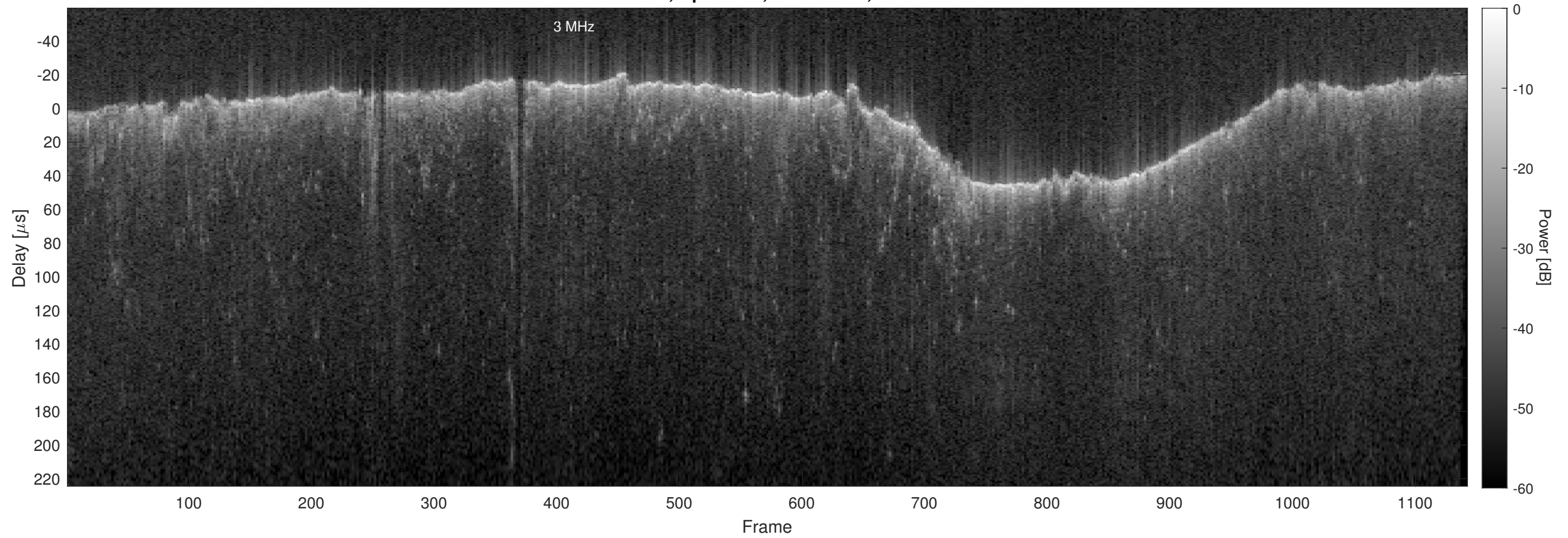
Orbit 15428, Optimized, No Window, Channel 2
