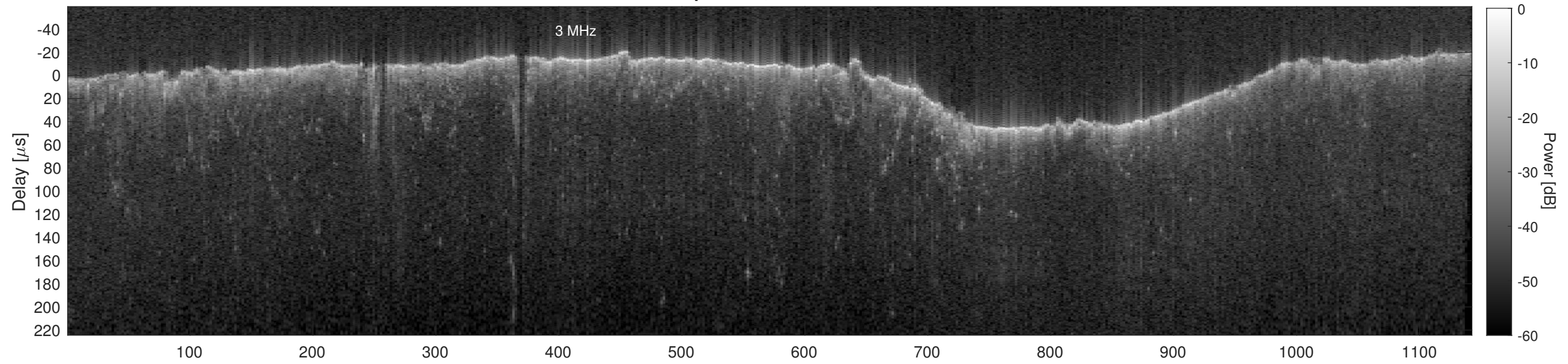
Orbit 15428, Cluttergram
