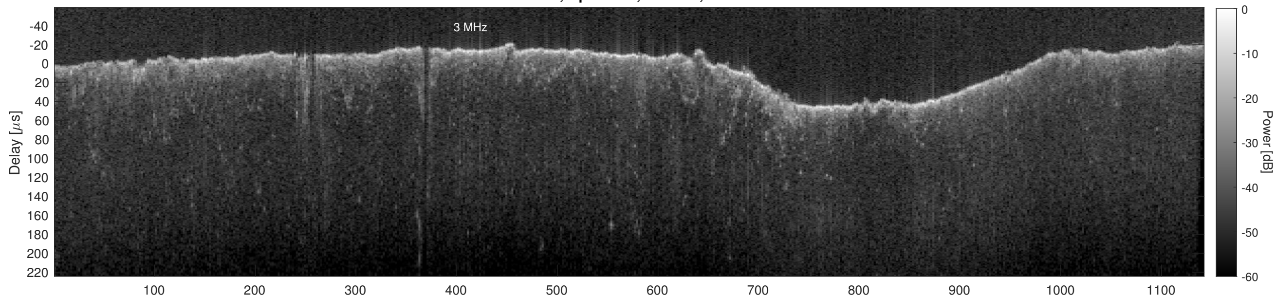
Orbit 15428, Cluttergram
