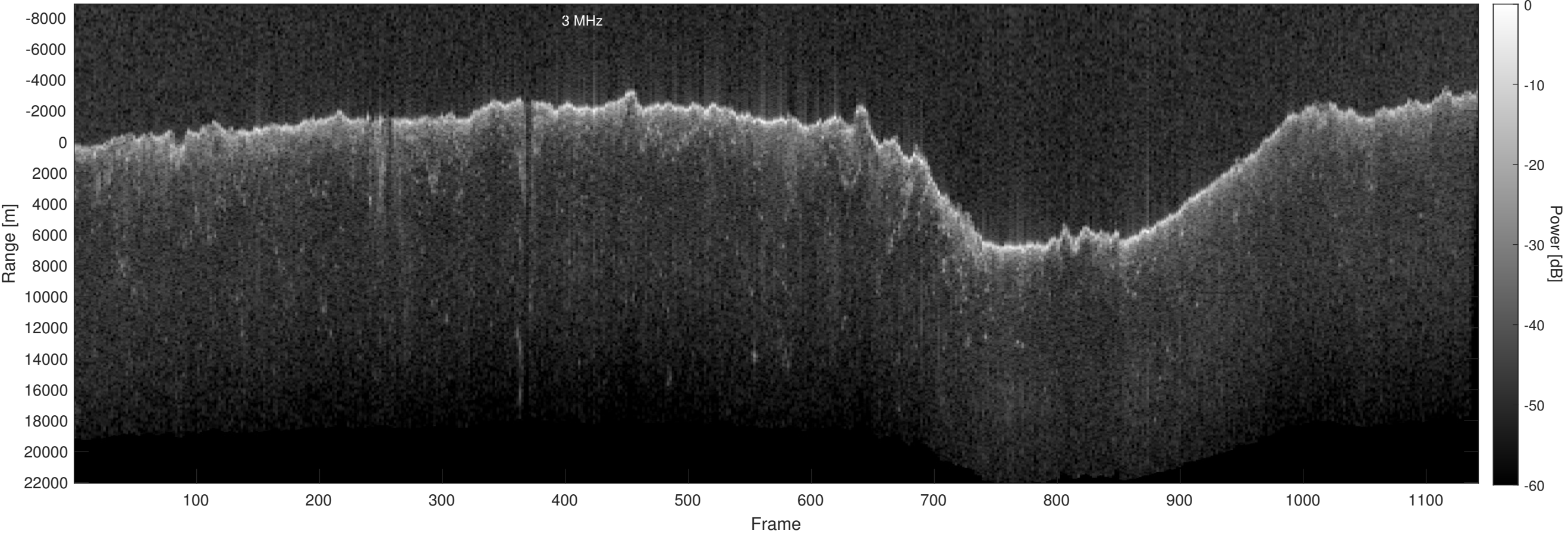
Orbit 15428, Optimized, Window, Depth-Corrected, Channel 2
