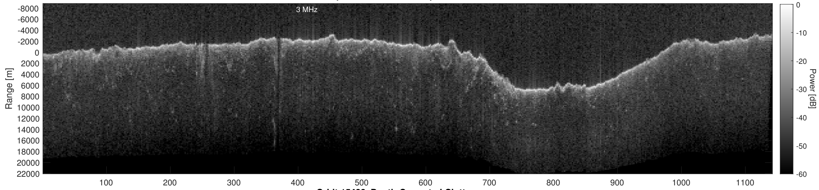
Orbit 15428, Depth-Corrected Cluttergram
