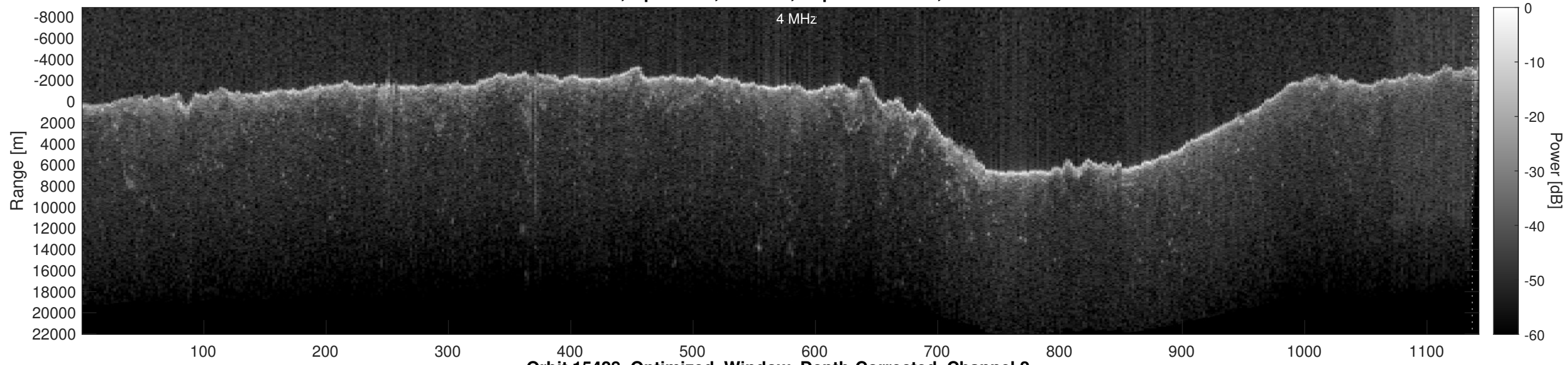
Orbit 15428, Optimized, Window, Depth-Corrected, Channel 2
