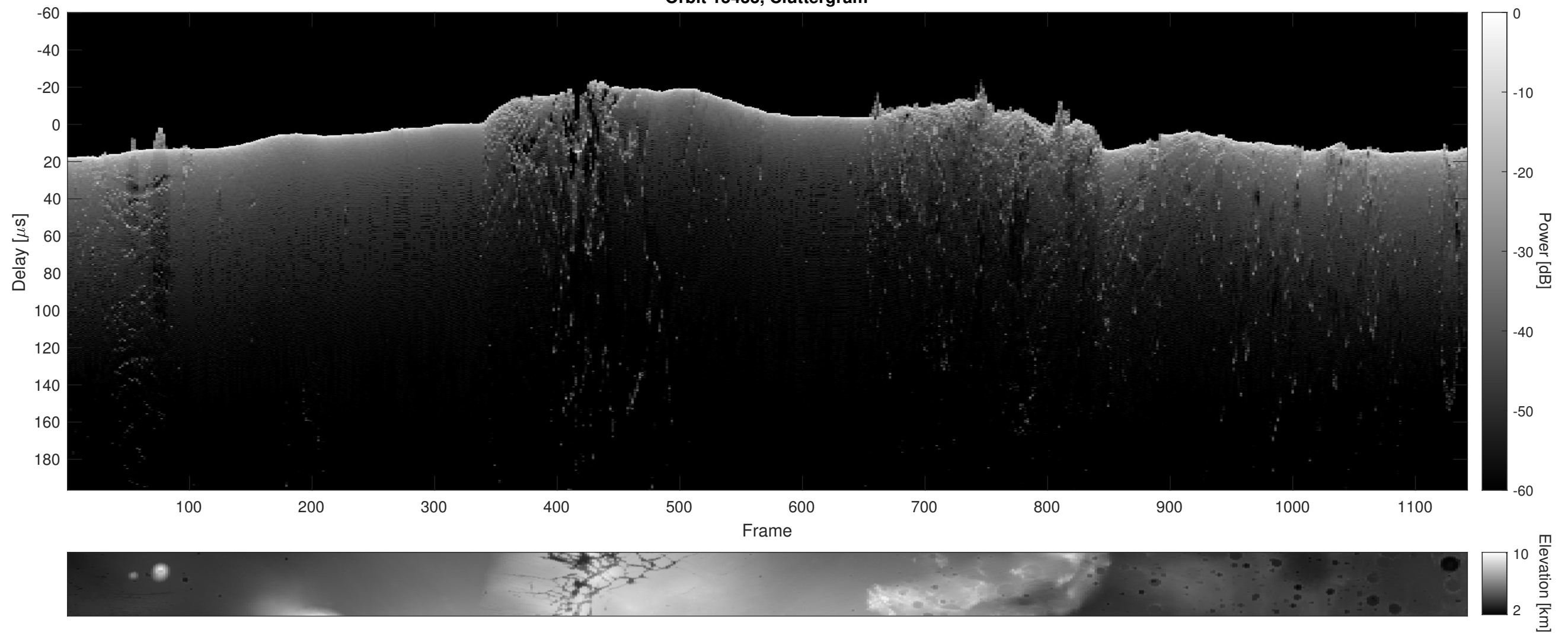
Orbit 15433, Cluttergram
