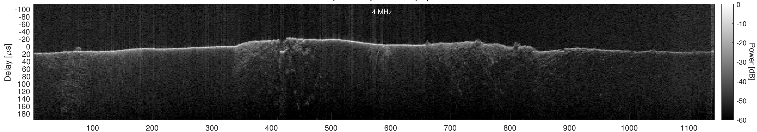
Orbit 15433, Cluttergram
