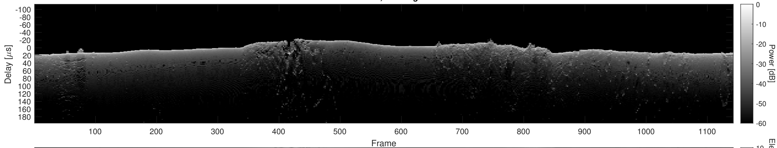
Orbit 15433, Cluttergram
