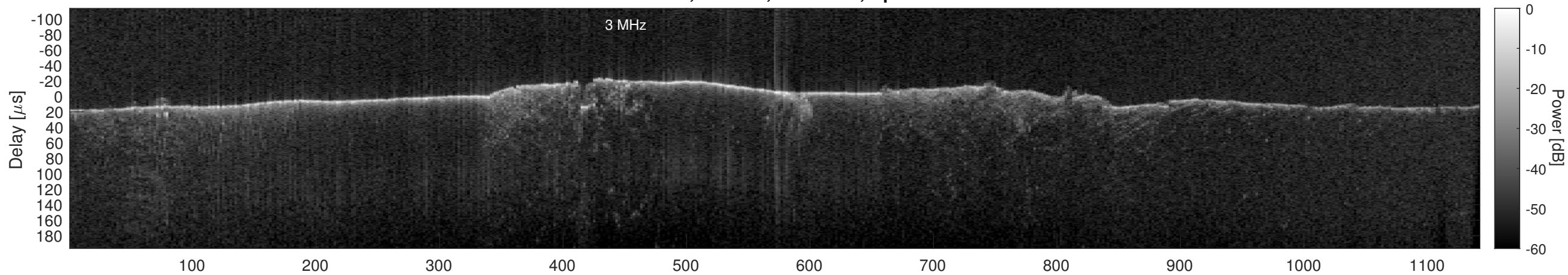
Orbit 15433, Cluttergram
