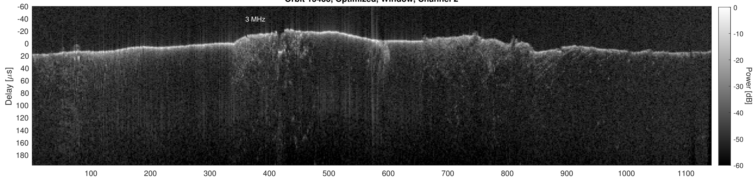
Orbit 15433, Cluttergram
