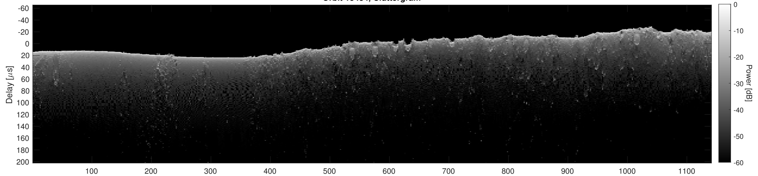
Orbit 15434, Cluttergram
