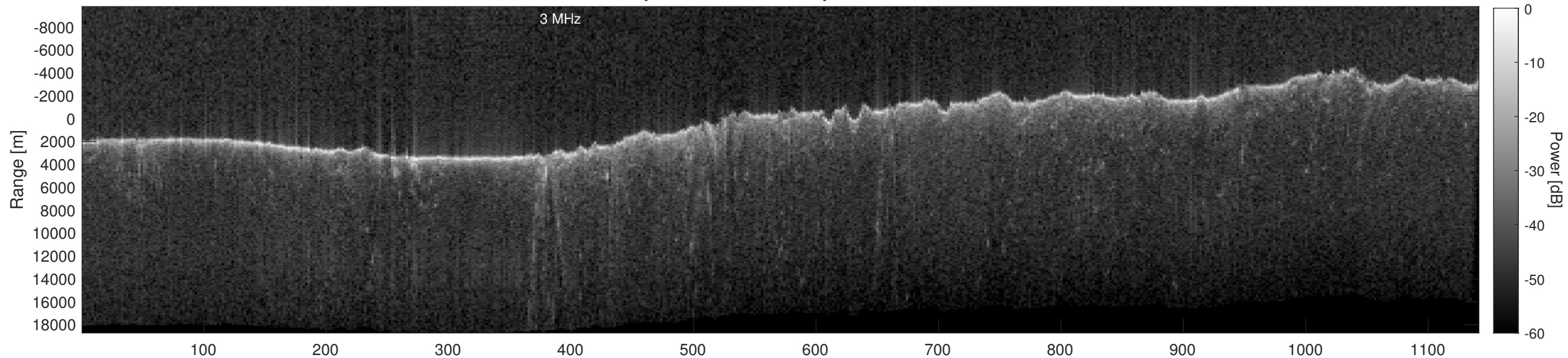
Orbit 15434, Depth-Corrected Cluttergram
