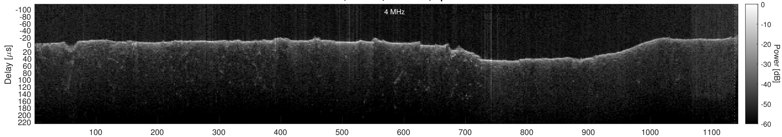
Orbit 15435, Cluttergram
