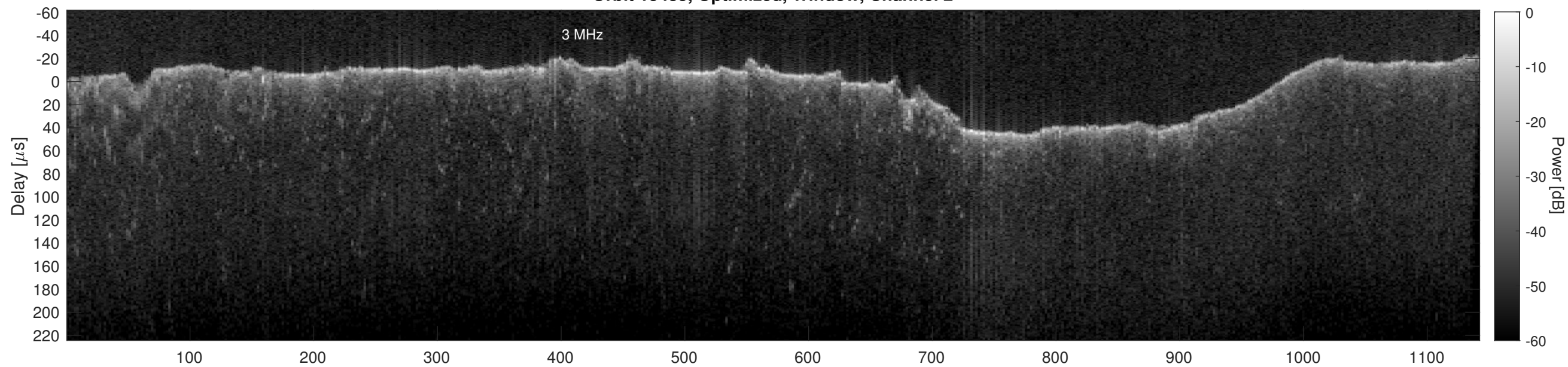
Orbit 15435, Cluttergram
