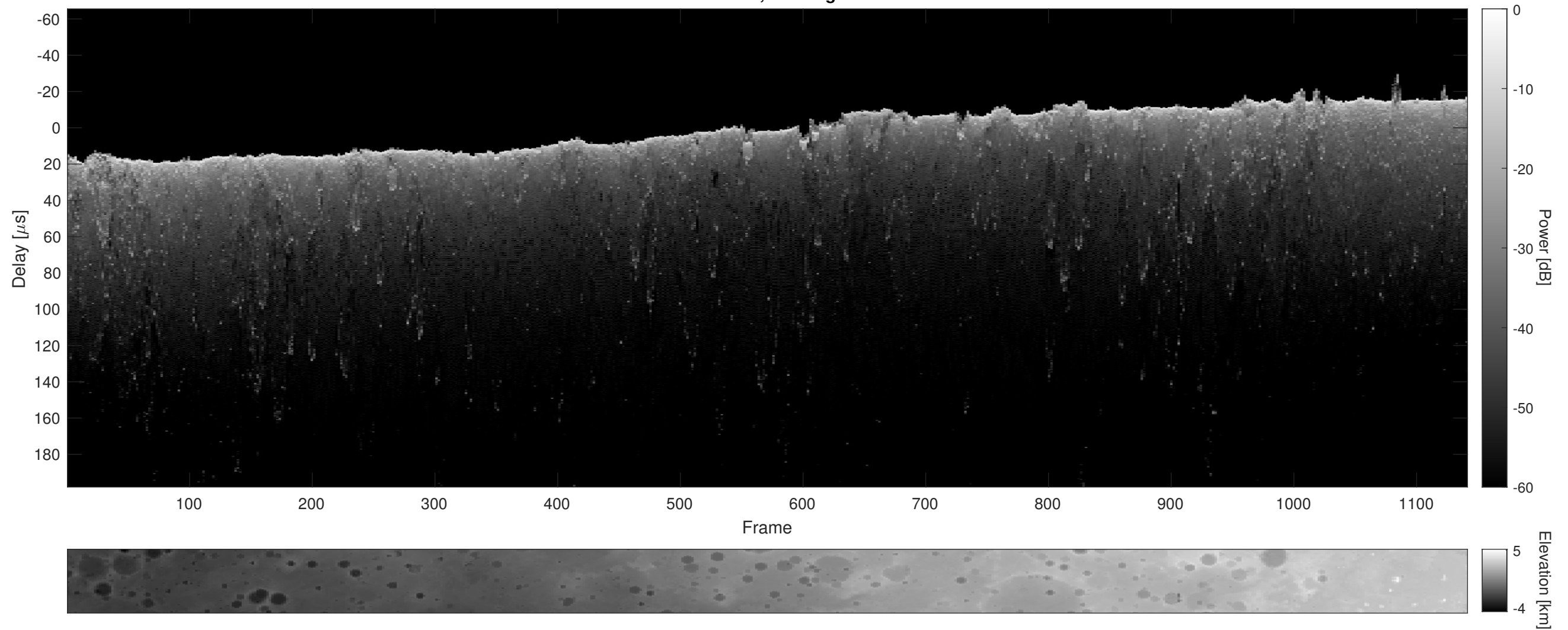
Orbit 15439, Cluttergram
