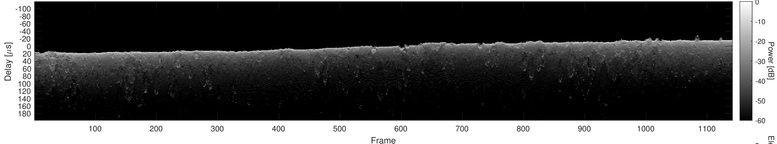
Orbit 15439, Cluttergram
