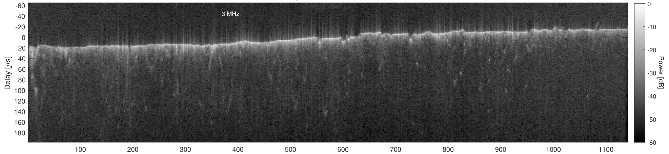
Orbit 15439, Cluttergram
