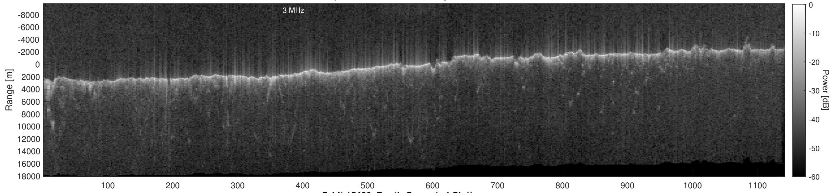
Orbit 15439, Depth-Corrected Cluttergram
