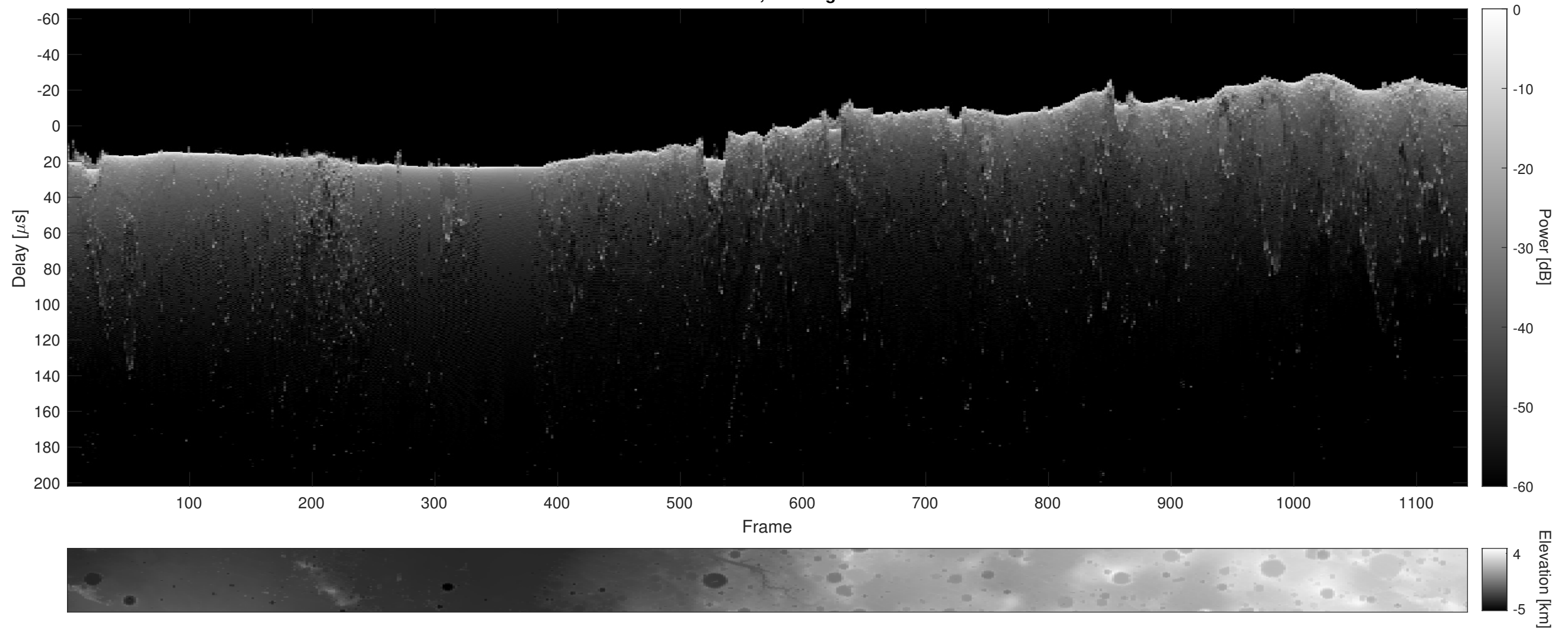
Orbit 15441, Cluttergram
