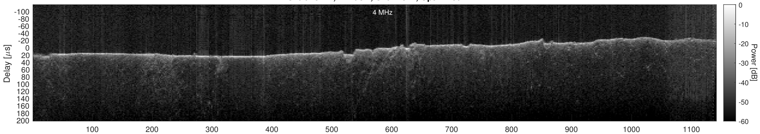
Orbit 15441, Cluttergram
