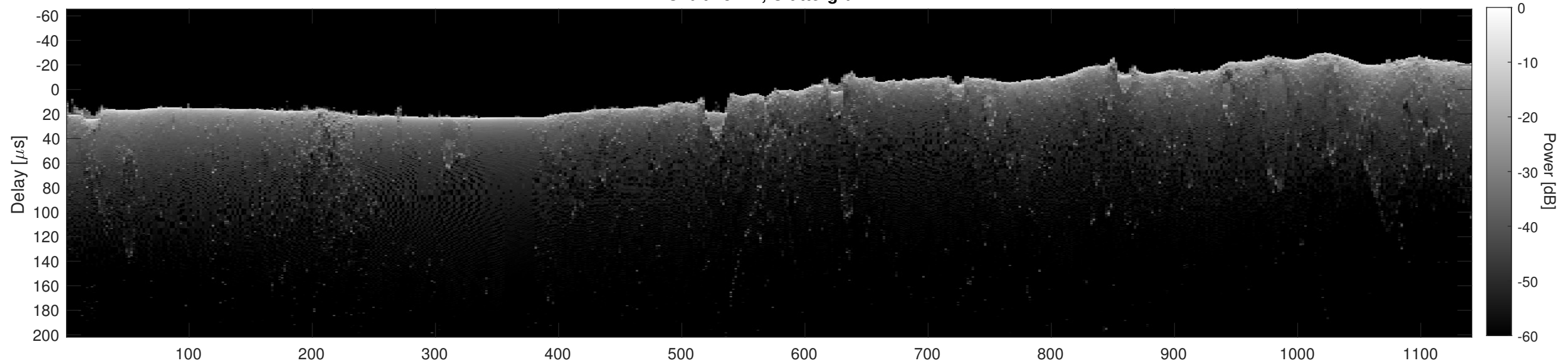
Orbit 15441, Cluttergram
