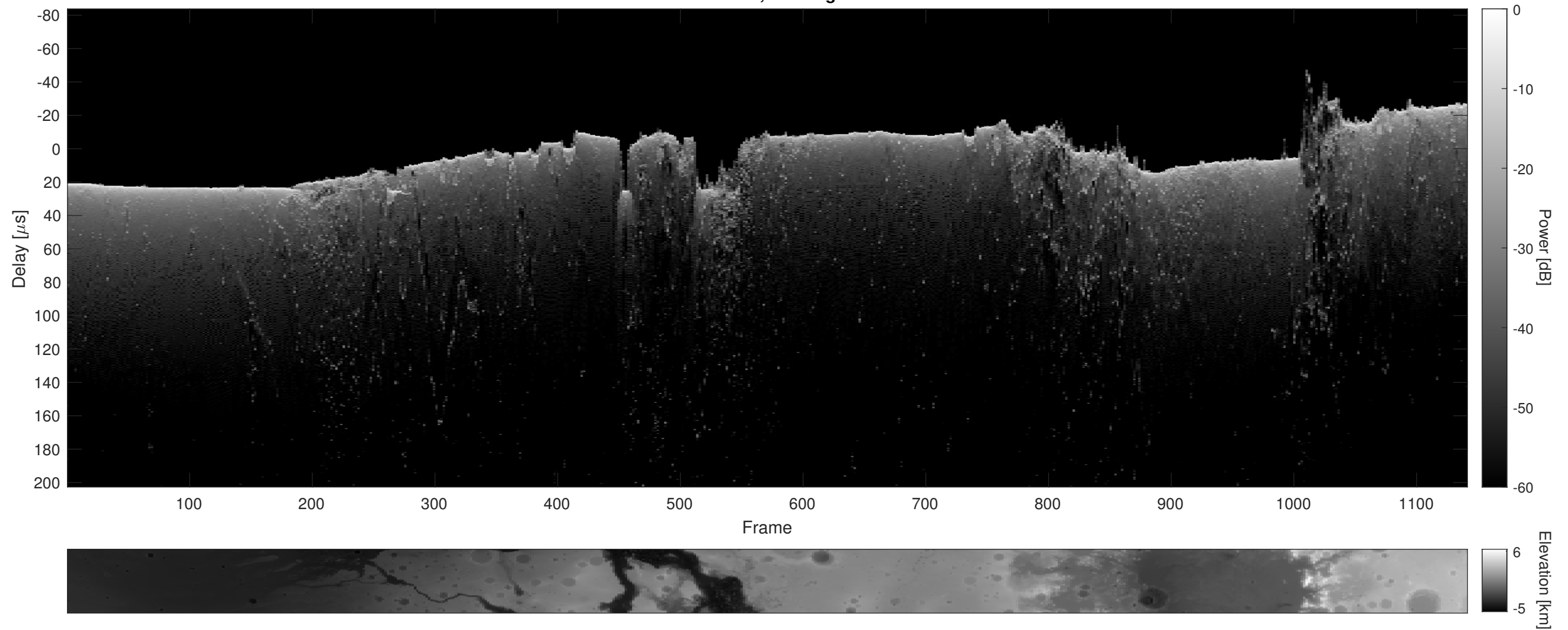
Orbit 15443, Cluttergram
