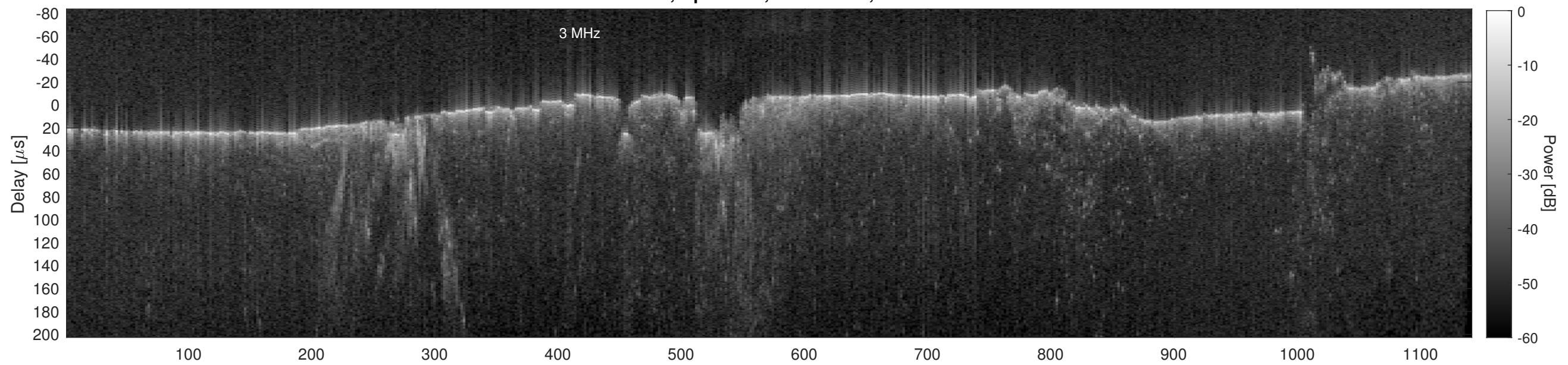
Orbit 15443, Cluttergram
