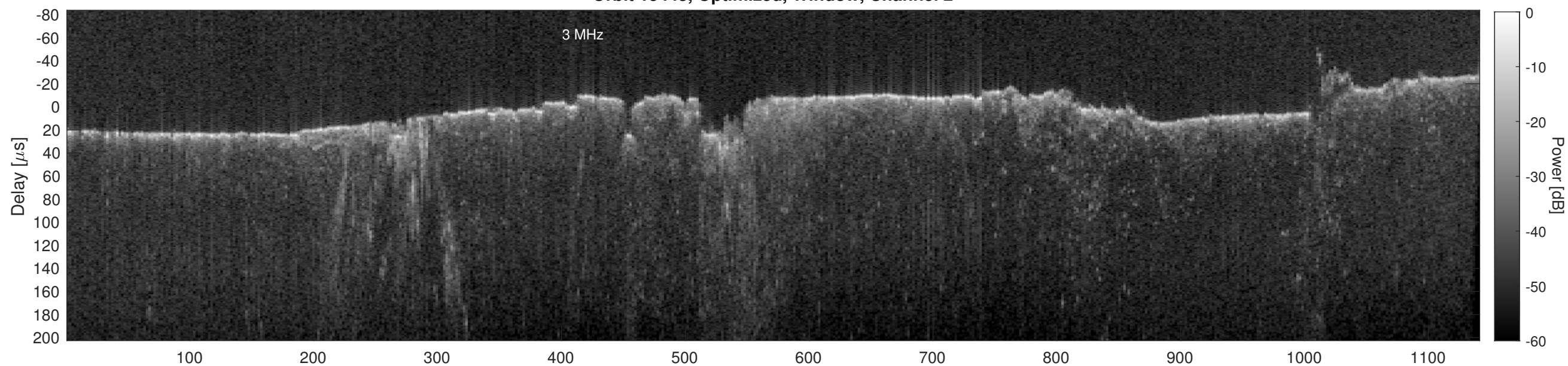
Orbit 15443, Cluttergram
