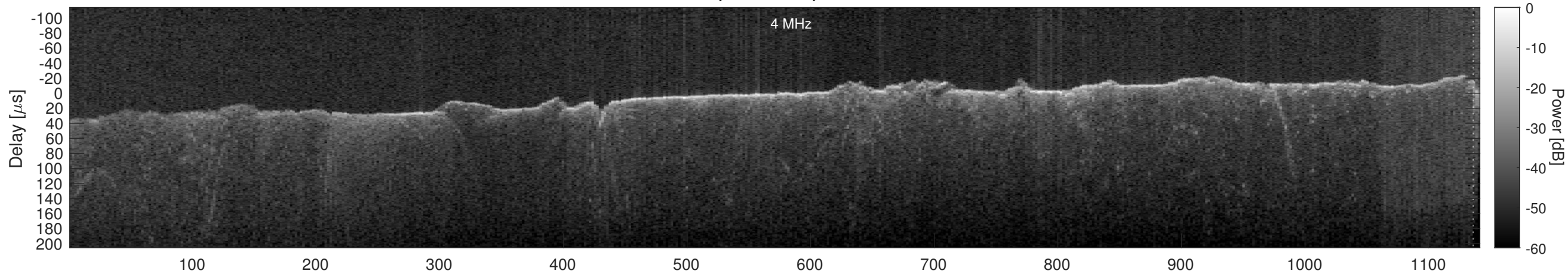
Orbit 15444, Window, Channel 1, Chapman
