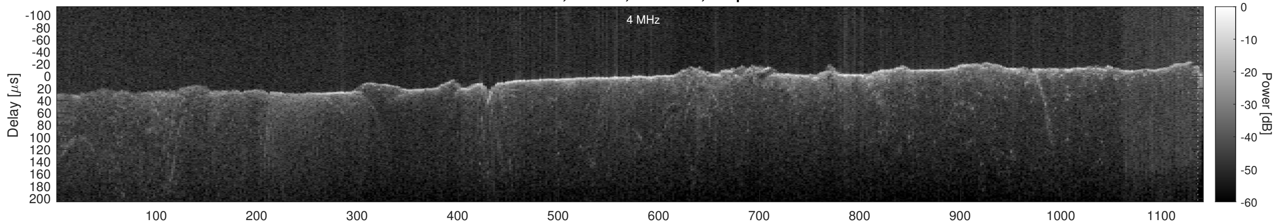
Orbit 15444, Window, Channel 1, Optimized
