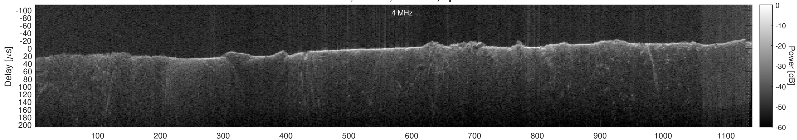
Orbit 15444, Cluttergram
