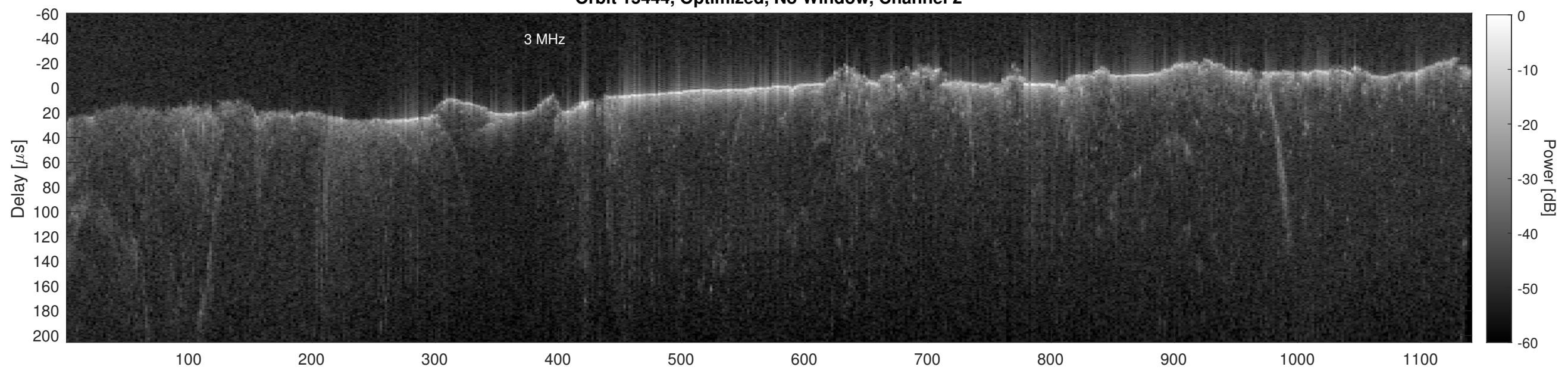
Orbit 15444, Cluttergram
