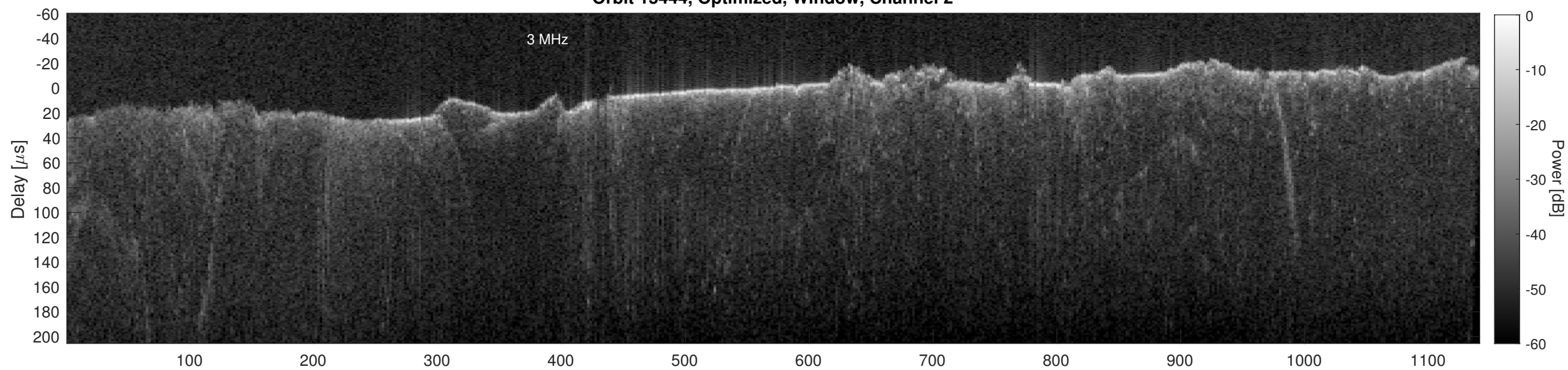
Orbit 15444, Cluttergram
