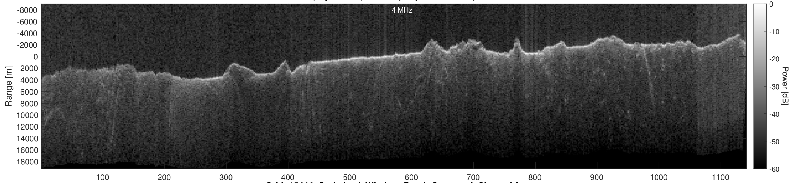
Orbit 15444, Optimized, Window, Depth-Corrected, Channel 2
