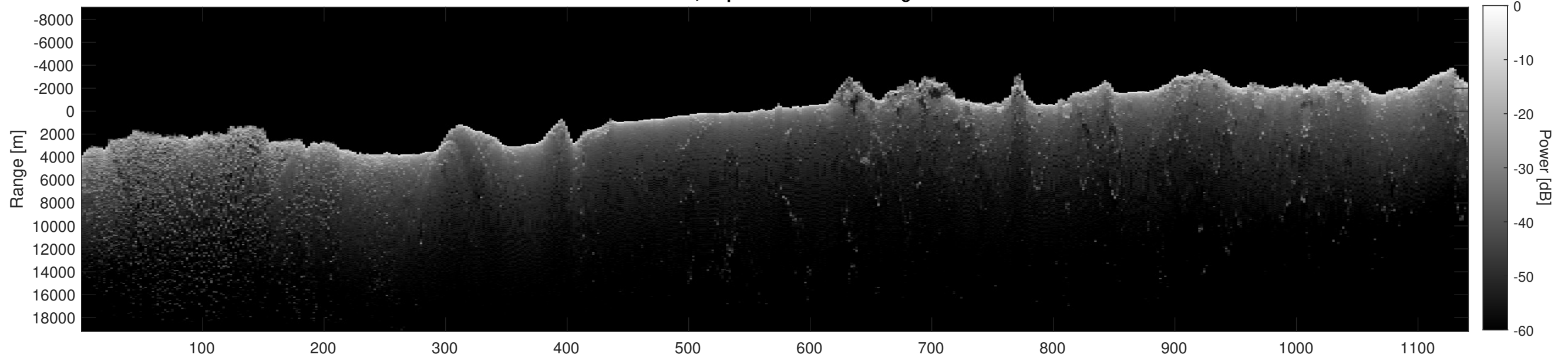
Orbit 15444, Depth-Corrected Cluttergram
