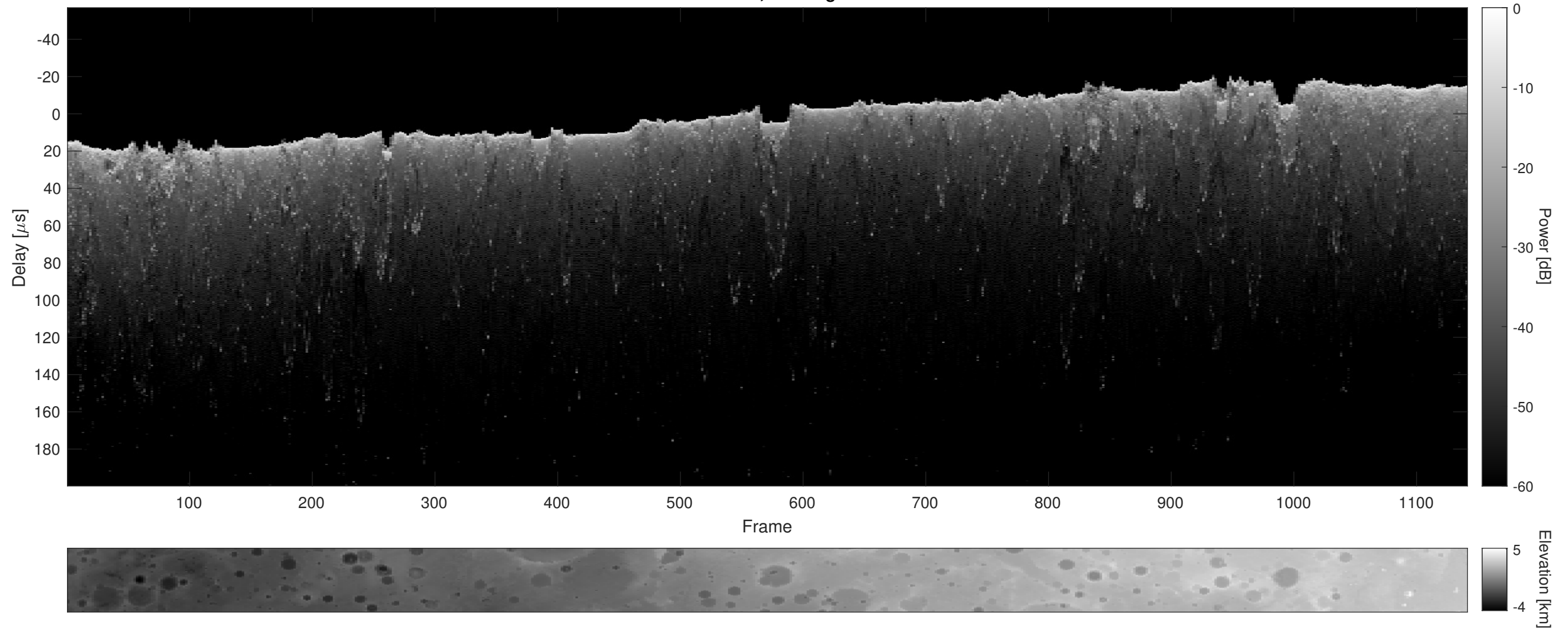
Orbit 15446, Cluttergram
