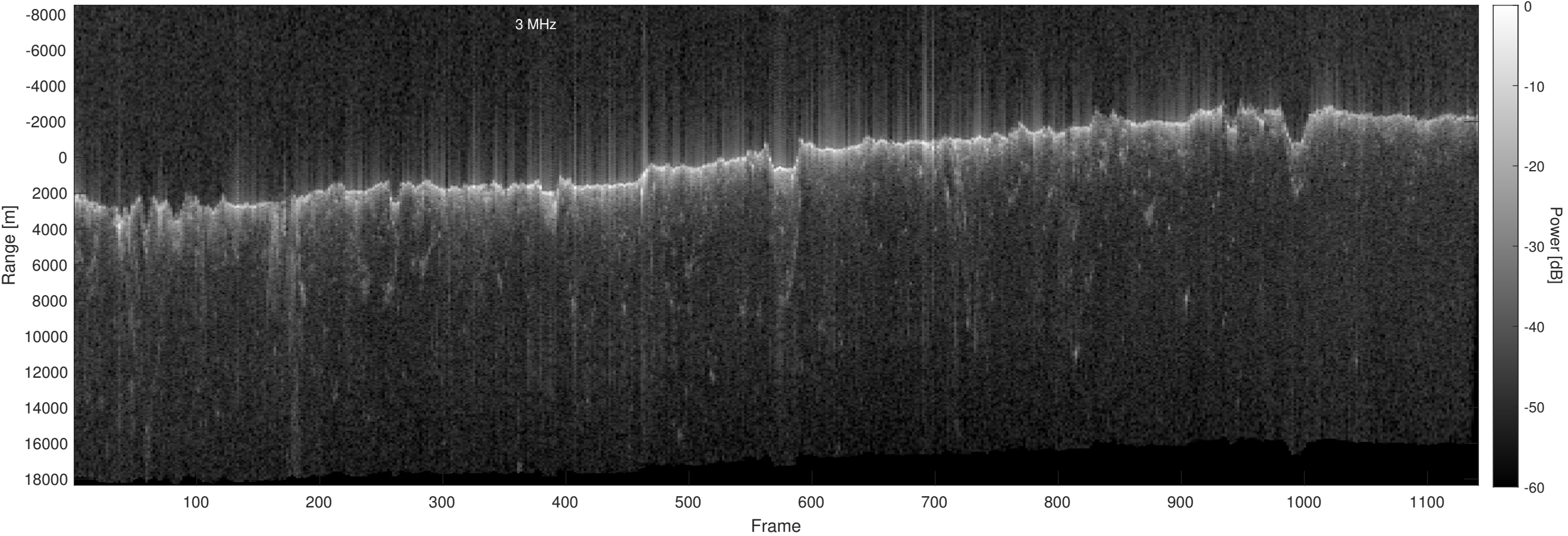
Orbit 15446, Optimized, No Window, Depth-Corrected, Channel 2
