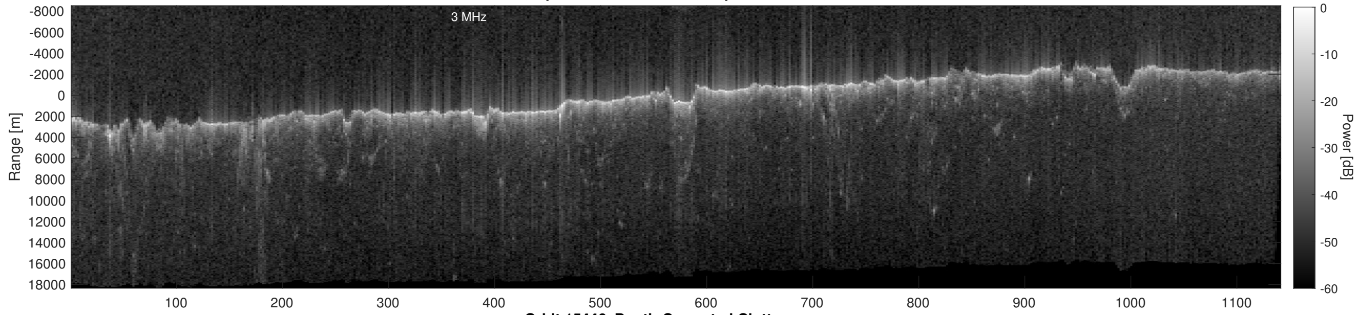
Orbit 15446, Depth-Corrected Cluttergram
