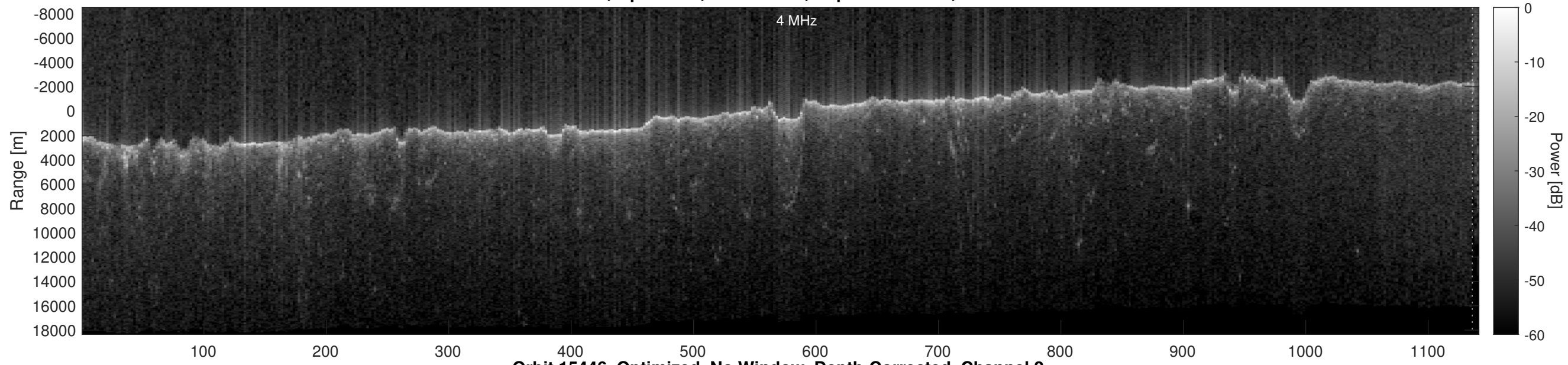
Orbit 15446, Optimized, No Window, Depth-Corrected, Channel 2
