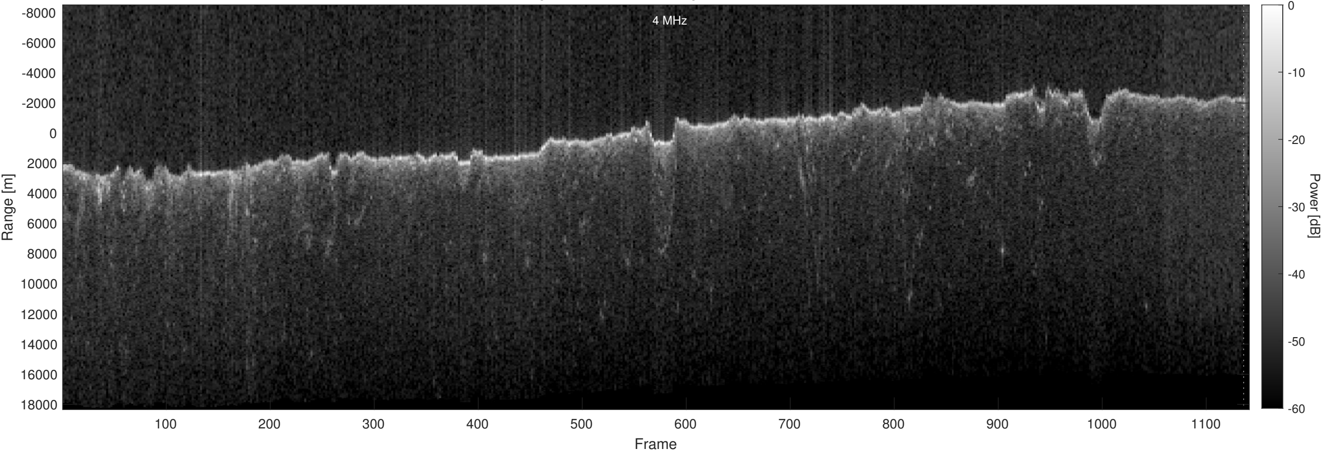
Orbit 15446, Optimized, Window, Depth-Corrected, Channel 2
