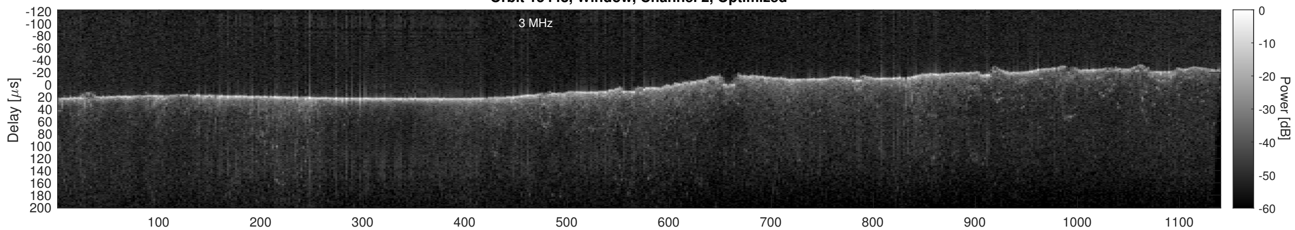
Orbit 15448, Cluttergram
