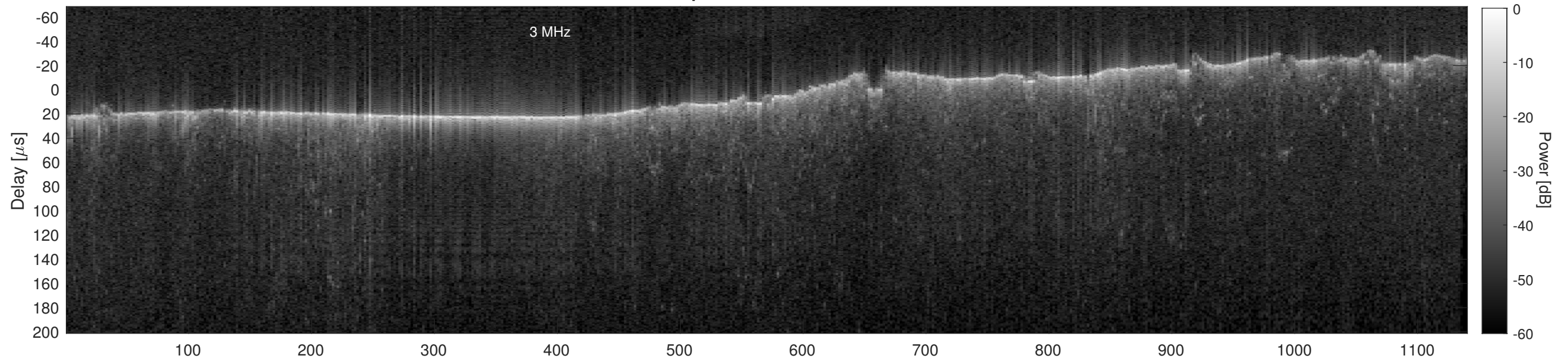
Orbit 15448, Cluttergram
