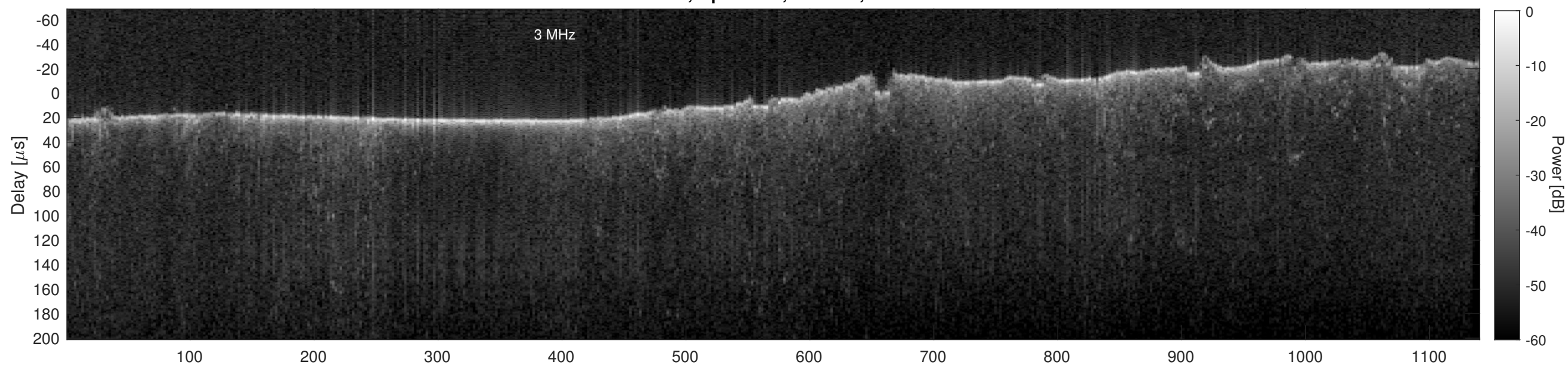
Orbit 15448, Cluttergram
