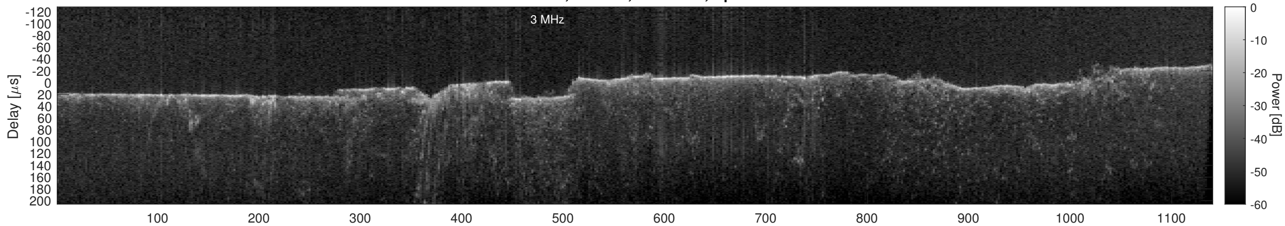
Orbit 15450, Cluttergram
