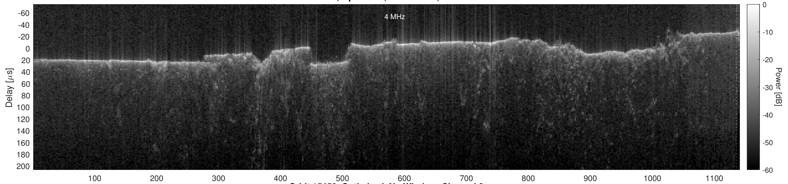
Orbit 15450, Optimized, No Window, Channel 2
