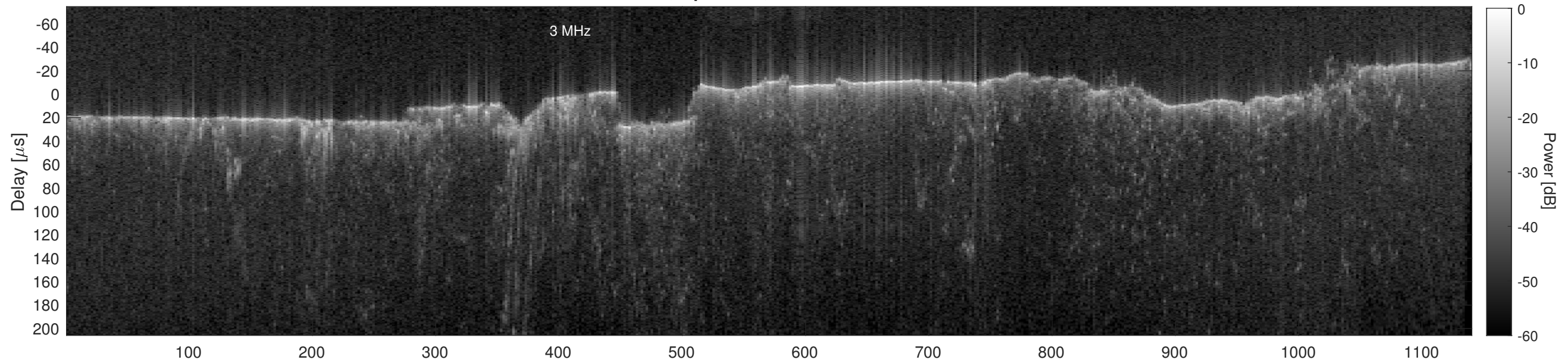
Orbit 15450, Cluttergram
