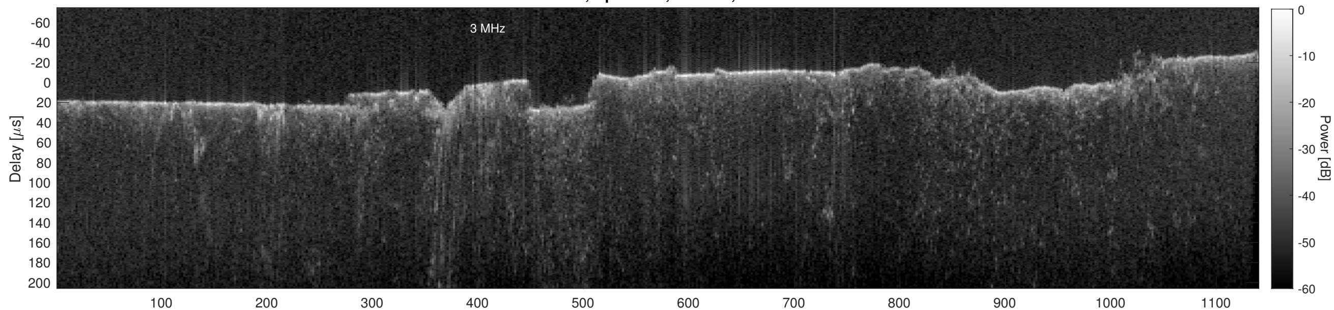
Orbit 15450, Cluttergram
