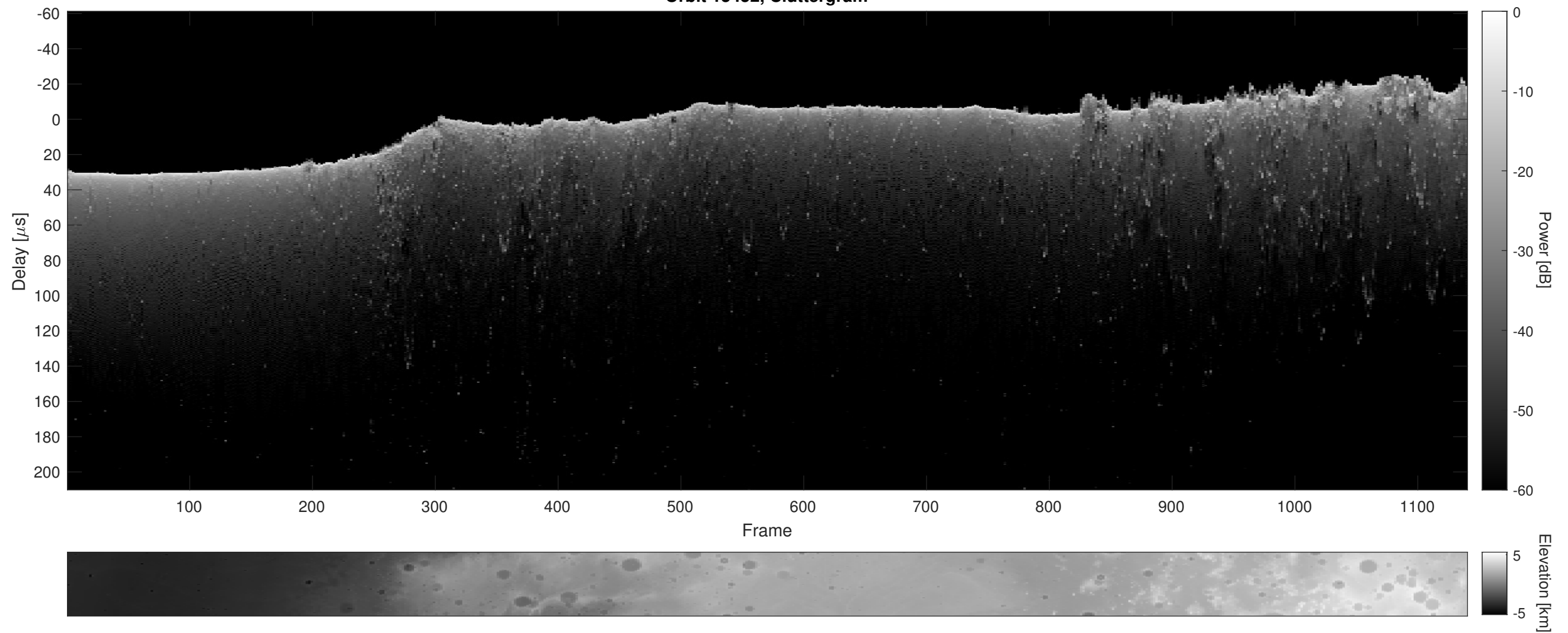
Orbit 15452, Cluttergram
