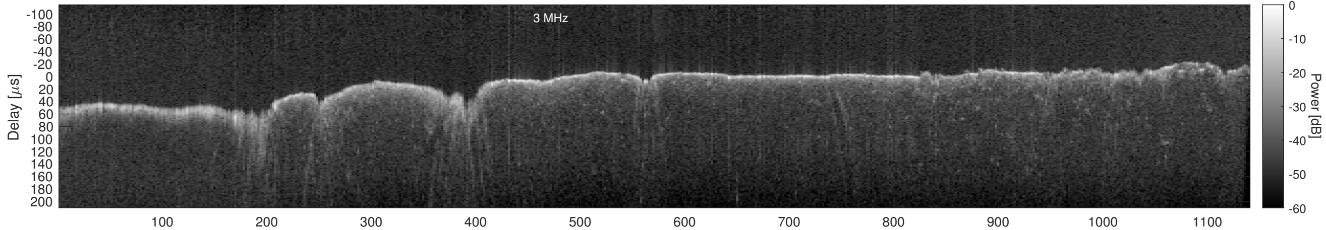
Orbit 15452, Window, Channel 2, Chapman
