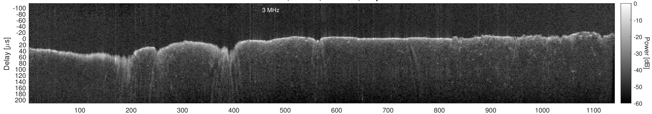
Orbit 15452, Window, Channel 2, Optimized
