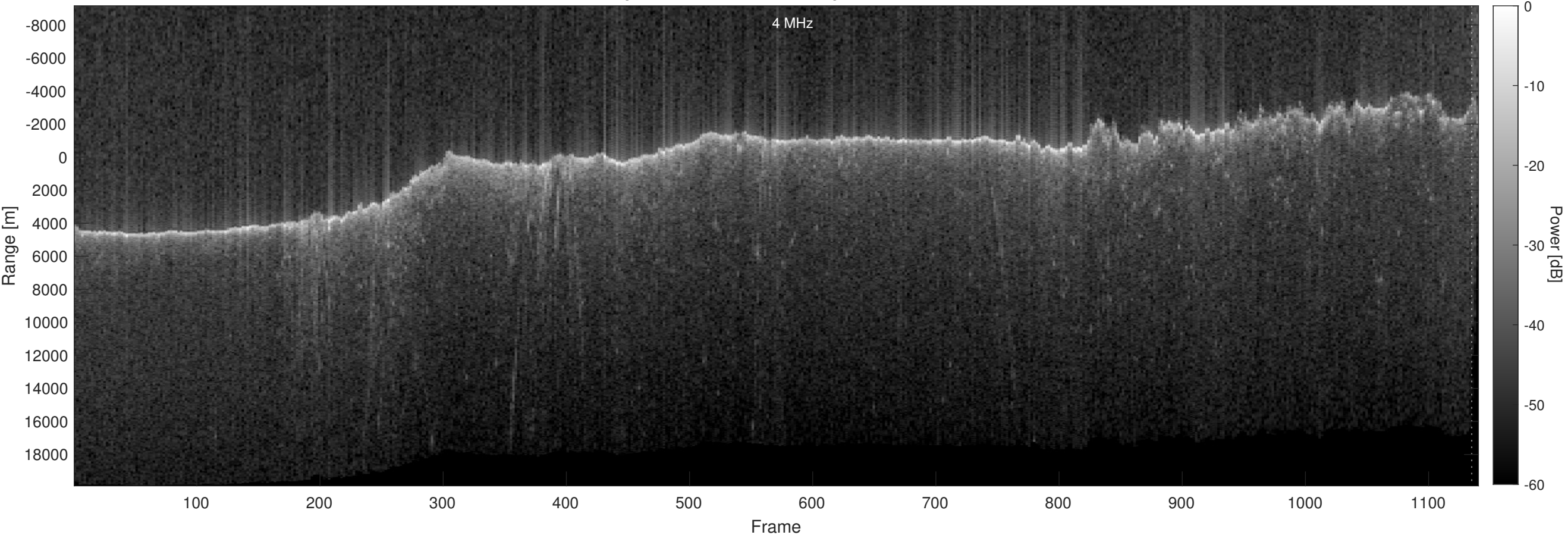
Orbit 15452, Optimized, No Window, Depth-Corrected, Channel 2
