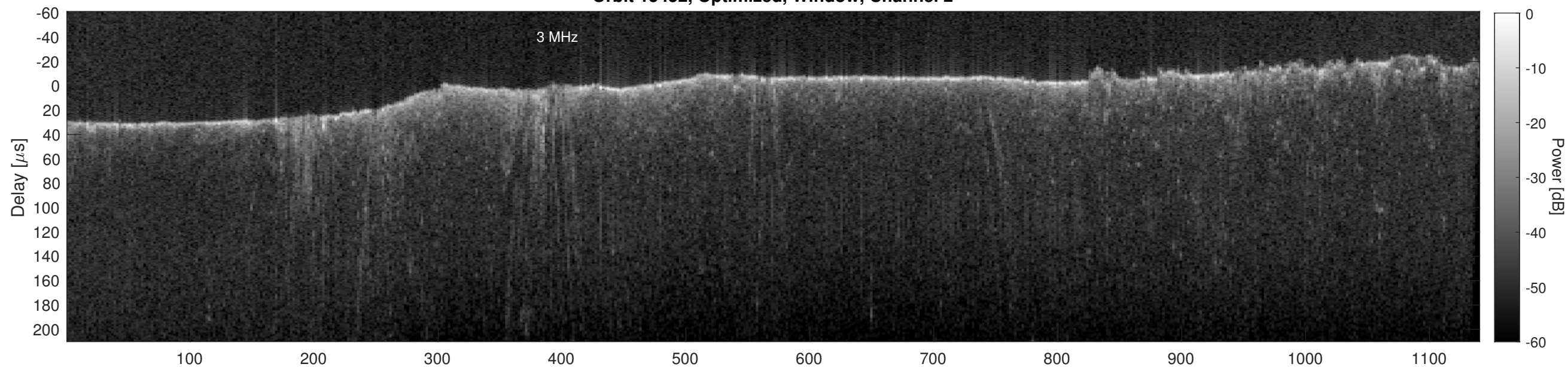
Orbit 15452, Cluttergram
