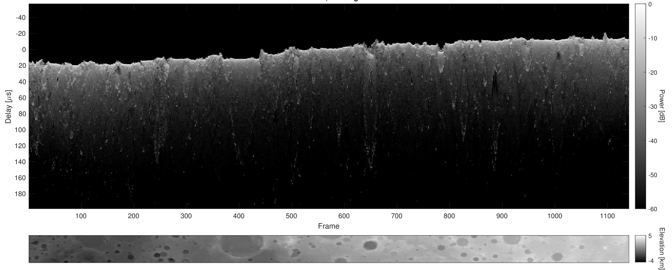
Orbit 15453, Cluttergram
