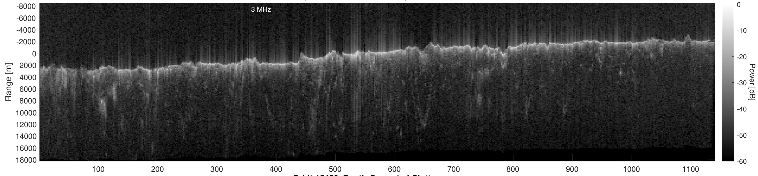
Orbit 15453, Depth-Corrected Cluttergram
