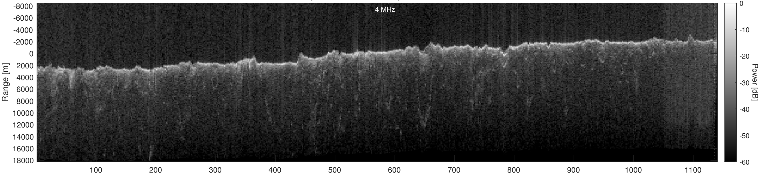
Orbit 15453, Optimized, Window, Depth-Corrected, Channel 2
