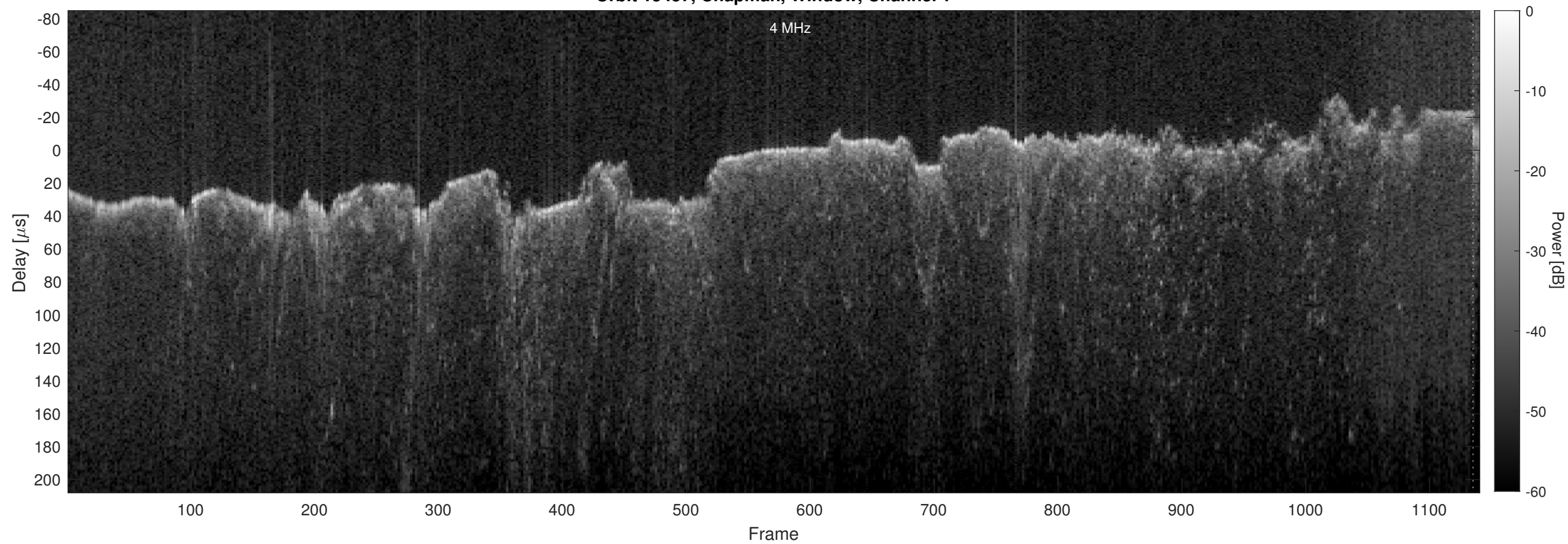
Orbit 15457, Chapman, Window, Channel 2
