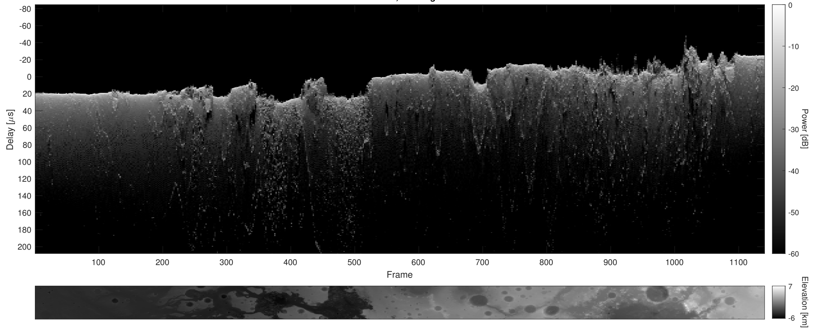
Orbit 15457, Cluttergram
