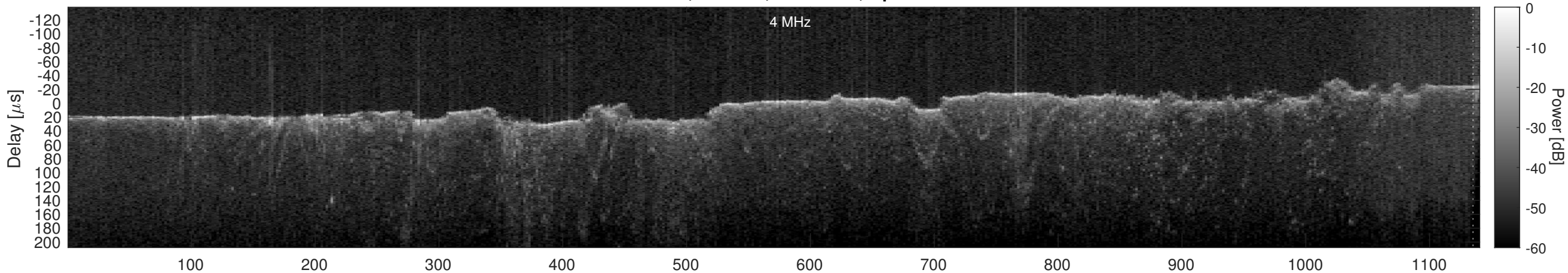
Orbit 15457, Cluttergram
