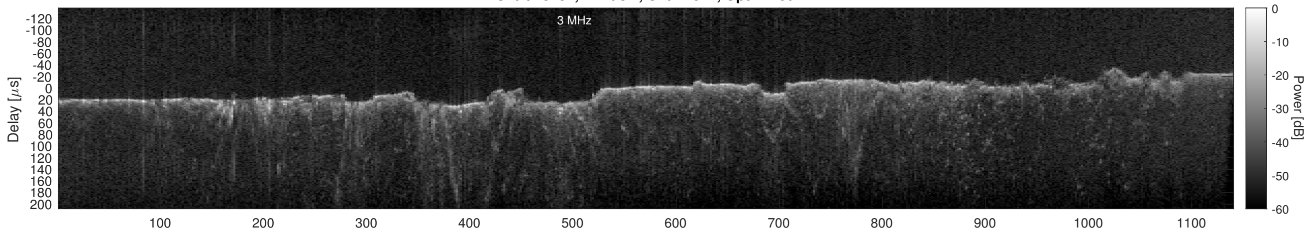
Orbit 15457, Cluttergram
