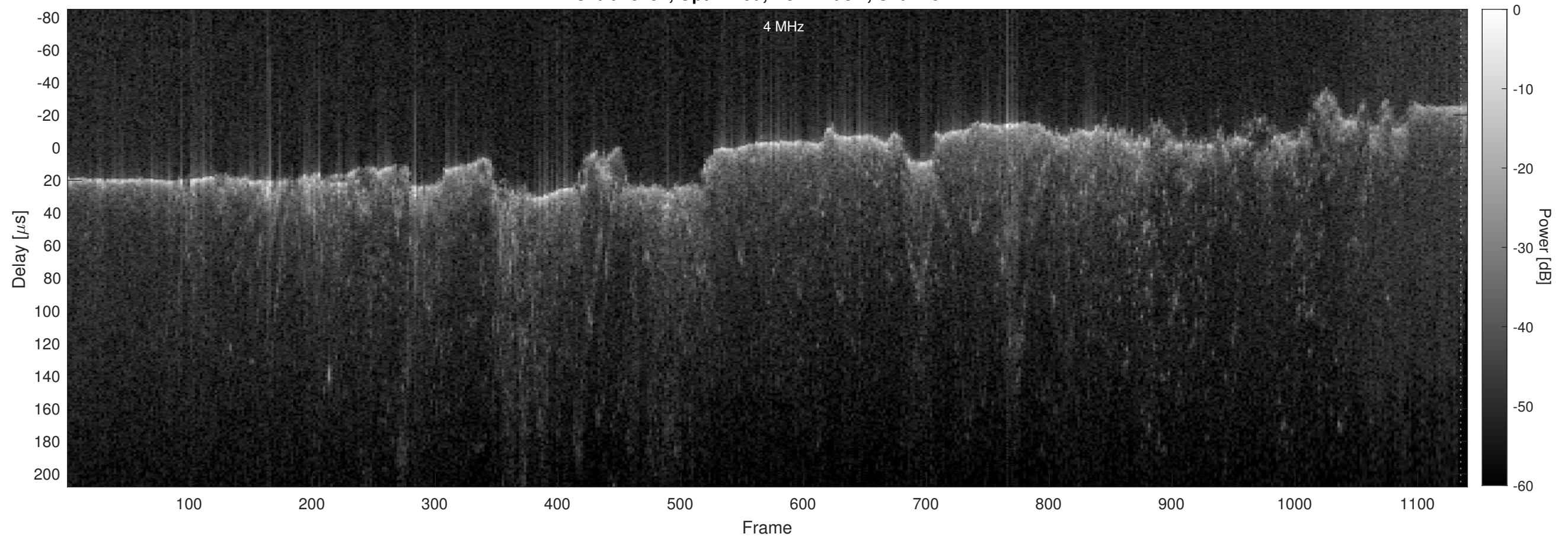
Orbit 15457, Optimized, No Window, Channel 2
