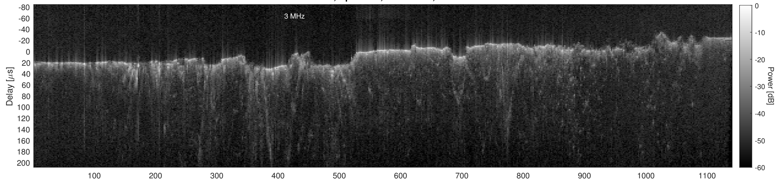
Orbit 15457, Cluttergram
